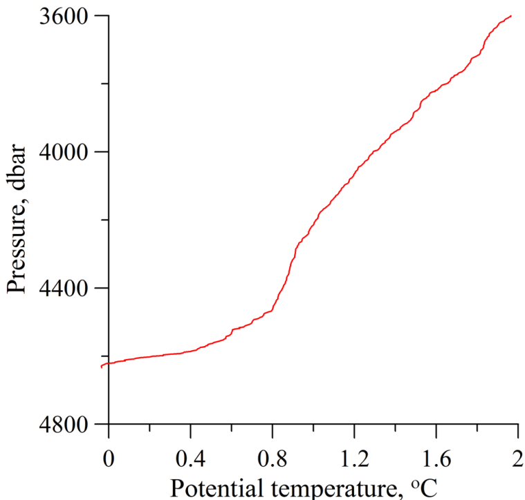
Figure 3. Profile of potential temperature at station 2527 at 26^{\circ}37.2' S, 33^{\circ}39.6' W. Near the bottom, a strong temperature gradient exists ( 0.8^{\circ}/150 m).
