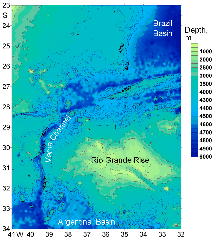
Figure 1. Bottom topography in the region of the Vema Channel based on ETOPO data.
