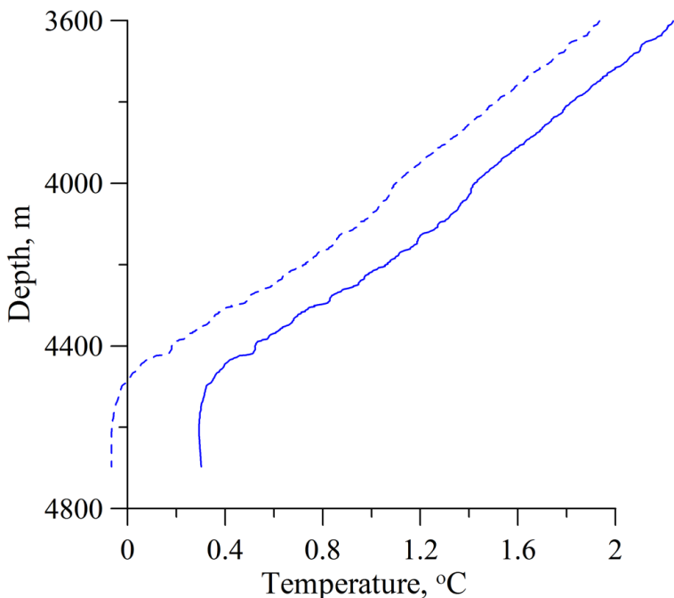
Figure 5. Solid curve shows in situ temperature profiles at station 2526 ( 26^{\circ}35.7' \text{ S} , 33^{\circ}51.6' \text{ W} , blue line). The dashed line shows the potential temperature.
