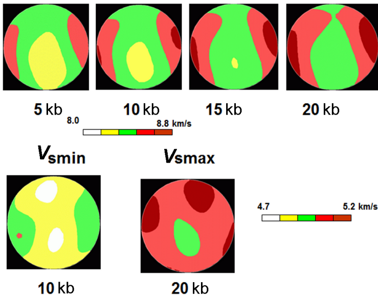
Figure 12. Calculated V_p and V_s of mantle xenolith CH-1 from the Bohemian Massif depending on pressure.
