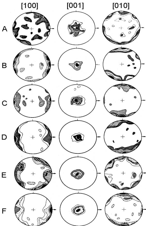
Figure 4. Olivine pole figures for six sections perpendicular to the long axis of xenolith CH-1 from the Bohemian Massif [ Grachev et al. , 1987]. The arrow in the right-hand part indicates the direction along which the thin sections were marked (Wulf's stereographic projection, upper hemisphere). All diagrams are based on data of 100 measurements.
