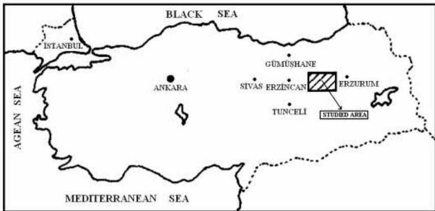
Figure 4. The location map of studied area.
