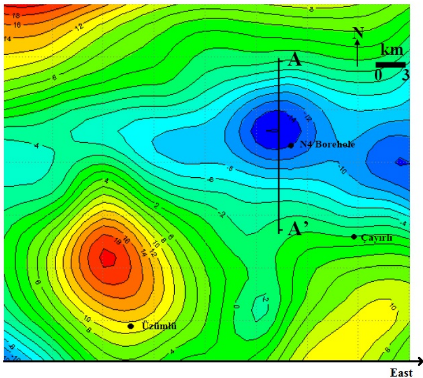
Figure 8. Residual gravity map of Erzincan-Cayirli (modified from MTA) and A-A' cross-section.
