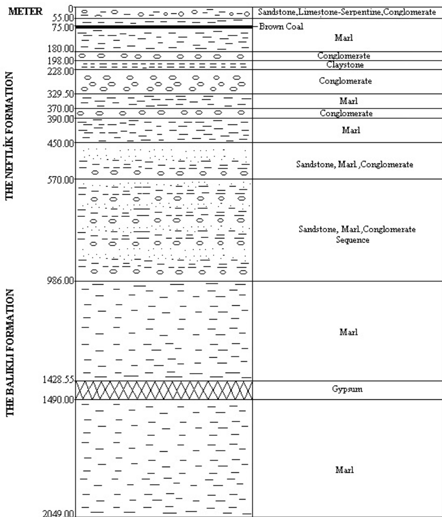
Figure 7. N4 Borehole cross-section (modified from [Demirmen, 1965]).
