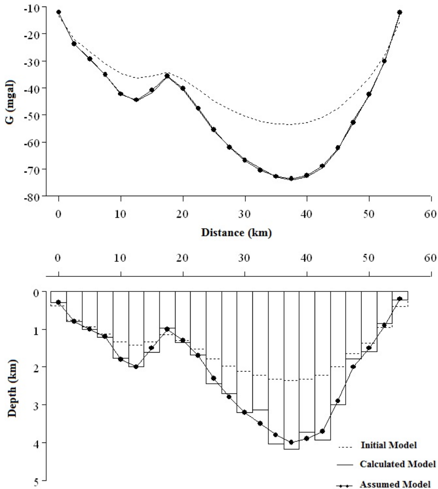
Figure 3. Results that are relating to noise added theoretical model.
