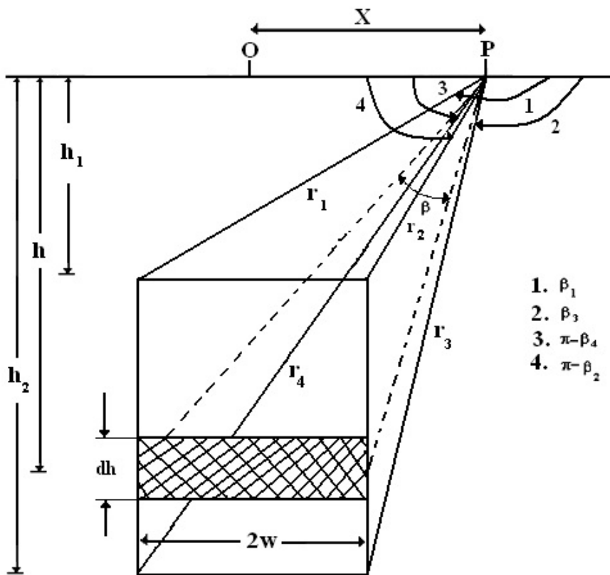
Figure 1. 2D vertical prism model ( O is the origin, P is the calculation point, h_1 and h_2 are the top and bottom depths, respectively) and its parameters.
