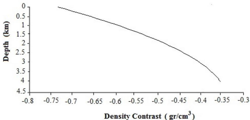
Figure 2. Correlation of density contrast-depth that is relating to the model.
