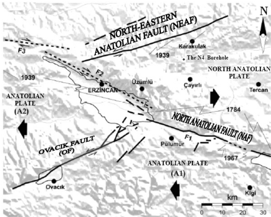
Figure 6. Effective faults that are around of Erzincan Basin and the Big Magnitude Earthquakes that are concerned with these faults (modified from [Kaypak and Eyidogan, 2002]).
