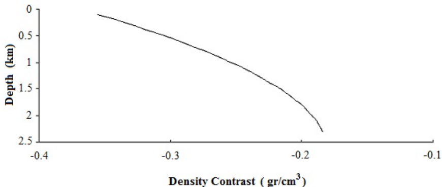
Figure 9. Correlation of density contrast-depth that is relating to the field model.
