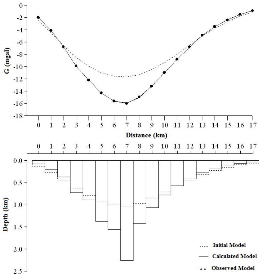
Figure 10. Results of the field model.
