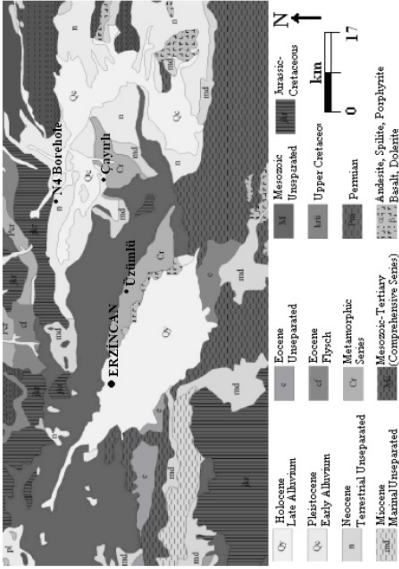
Figure 5. Geological map and studied area (modified from [Kaypak and Eydogan, 2002]).
