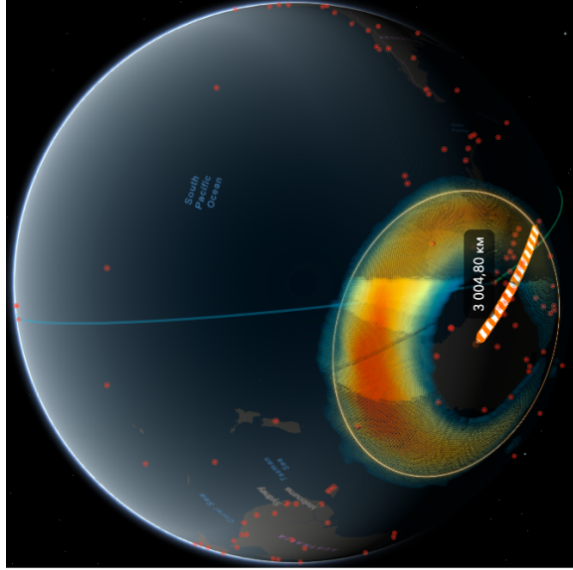
Figure 2. Visualization of auroras for the Northern (a) and Southern (b) hemispheres. An orange-white strip shows the option to measure the distance on the globe between any selected points.
