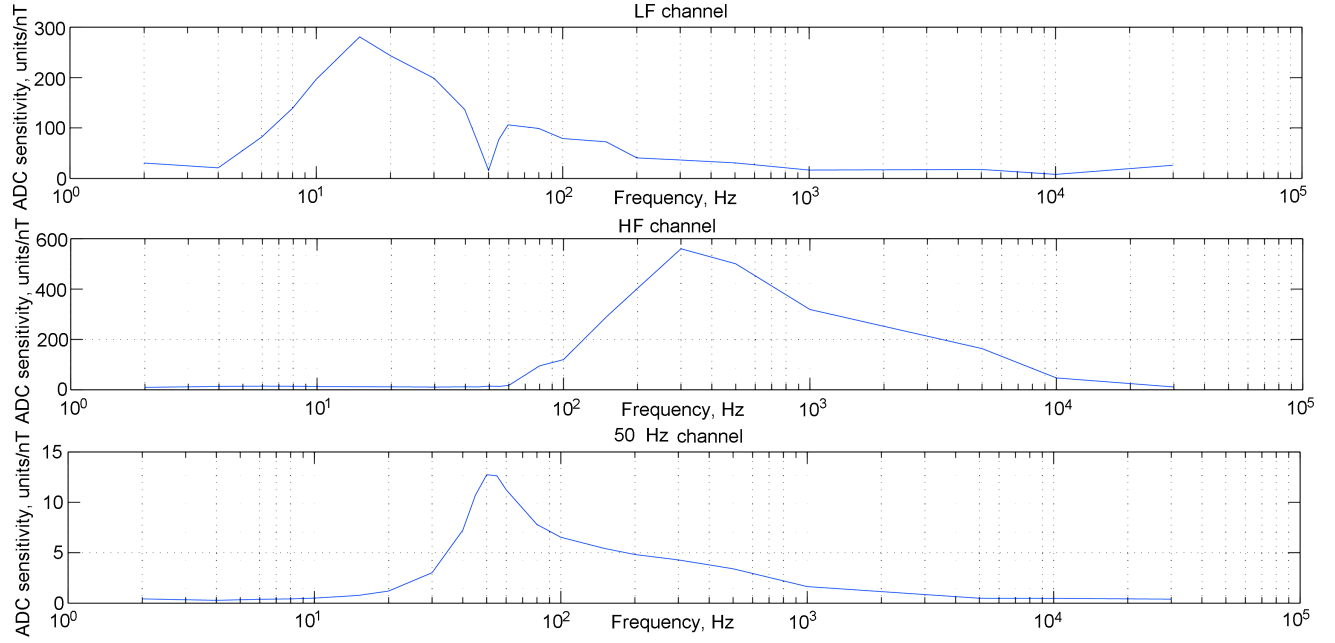
Figure 6. Amplitude-frequency response of the channels according to the results of calibration measurements.
