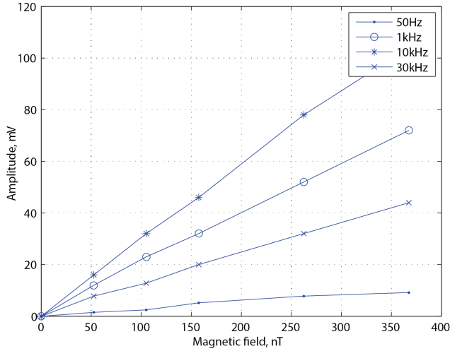
Figure 2. Characteristics of the induction sensor of the noise-meter: results of the tests.
