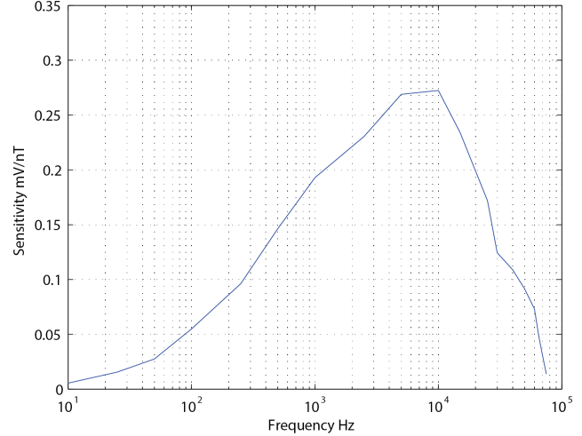
Figure 3. Characteristics of the induction sensor of the noise-meter: amplitude-frequency response.
