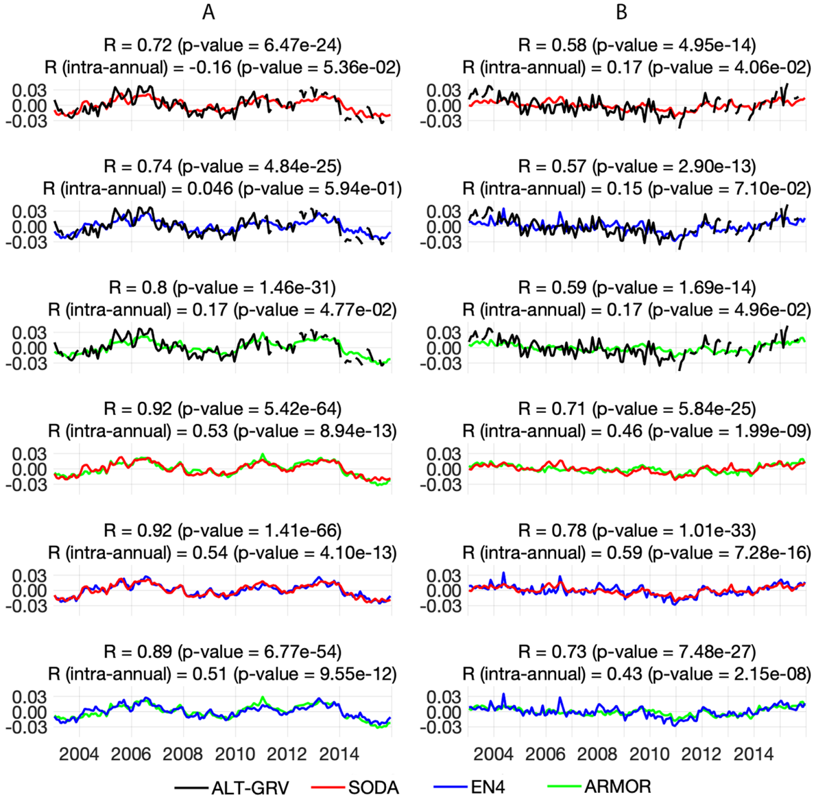
Figure 8. Time series of the steric sea-level fluctuations ( m ) averaged over area A (left column) and area B (right column). The linear trends and seasonal variability are removed.
