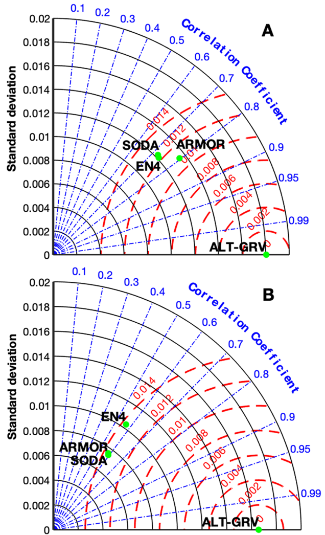
Figure 7. Taylor diagram displaying a statistical comparison with observations of the spatially averaged ALT-GRV, ARMOR, EN4, and SODA datasets for the area A and B.
