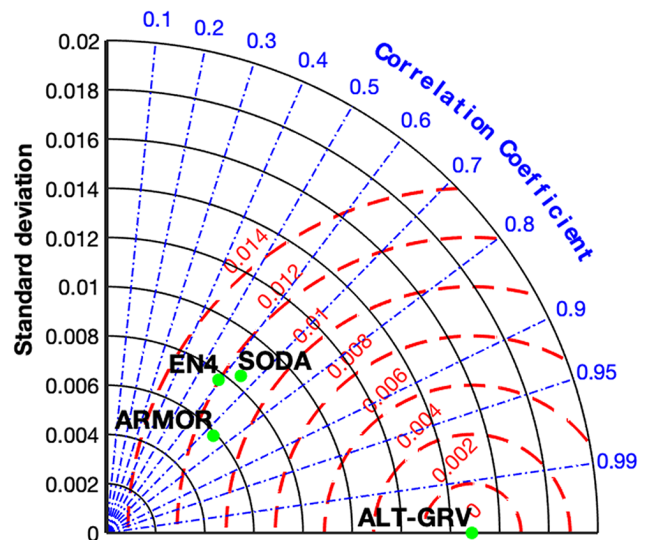
Figure 4. Taylor diagram displaying a statistical comparison with observations of the spatially averaged ALT-GRV, ARMOR, EN4, and SODA datasets for the study area.
