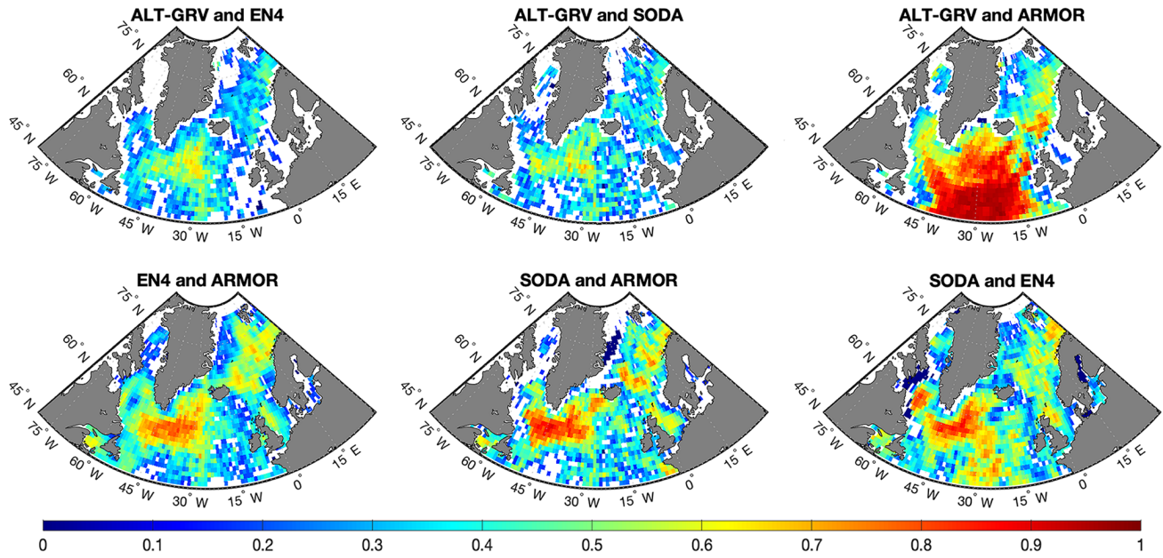
Figure 3. Spatial distribution of the correlation coefficients between the data sets. The linear trends and seasonal variability are removed.
