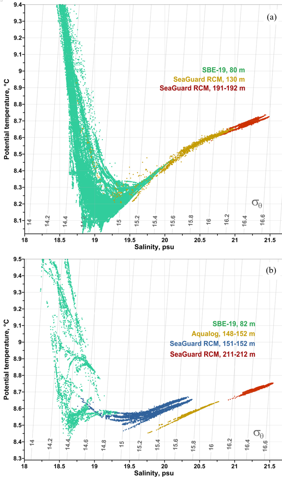
Figure 8. T - S diagram for the BBL according to the following data: a) SeaBird 19plus at 80 m (green dots), SeaGuard at 130 m (yellow dots) and 192 m (red dots); b) SeaBird 19plus at 82 m (green dots), SeaGuard at 152 m (blue dots) and 212 m (red dots), Aqualog at 152 m (the installation depth is 220 m, only the data from 152 m are used; yellow dots).
