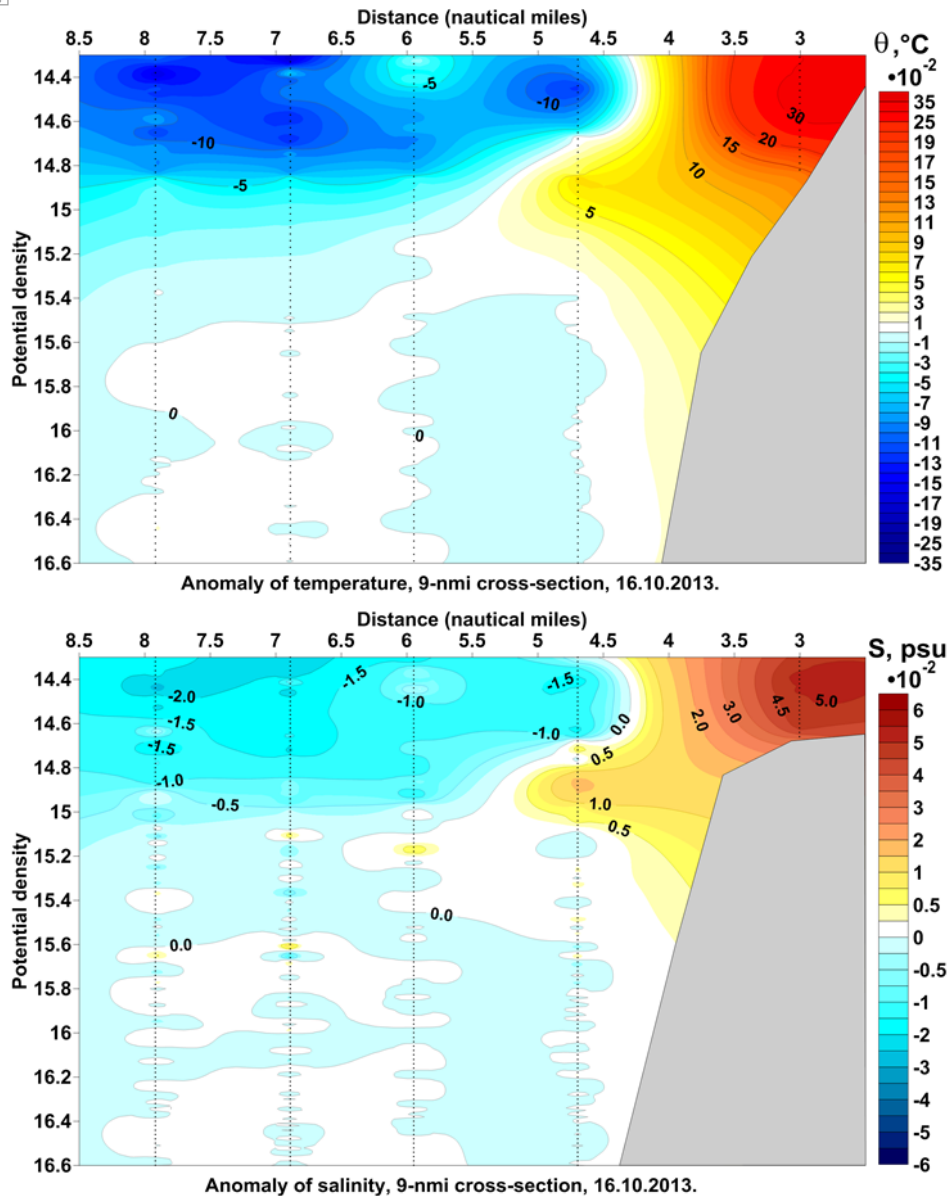
Figure 9. A thermohaline front, separating the warmer and more saline shelf water from the colder and less saline water above the continental slope.
