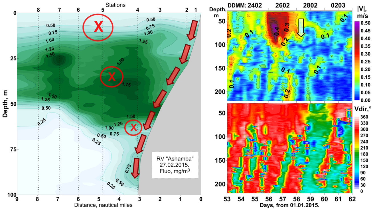
Figure 1. An intense northwestern current, which resulted in a water descent down the slope (right); its effect on a chlorophyll-a rich water, as observed during the ecological monitoring on a 9-nmi cross-section (left).
