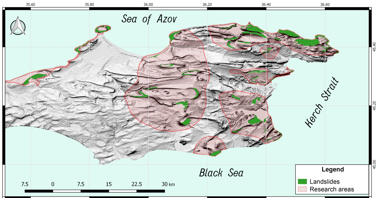
Figure 2. Map of the research areas and landslide locations.
