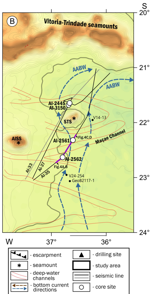
Figure 1. (B) Regional seafloor topography of the study area with direction of the AABW current and location of cores and seismoacoustic profiles. Bold purple lines indicate fragments of seismic profile AI-35 shown in Figure 4.
