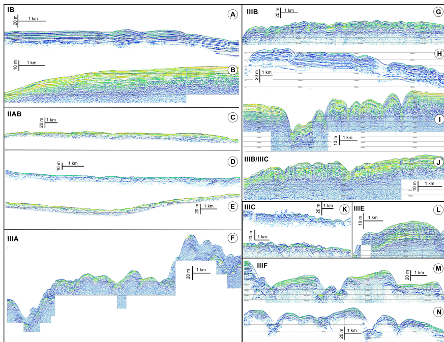
Figure 2. Seismic facies types distinguished in seismic sections (based on classification by Damuth and Hayes [1977]).
