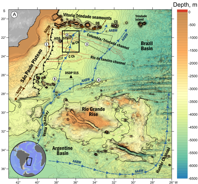
Figure 1. (A) Bathymetric map of the South Brazilian continental margin with directions of AABW and NADW currents, location of DSDP 515 drilling site and locations of main contourite, turbidite and mixed sedimentary systems (1 – São Tomé turbidite system [Viana et al. , 2003; Gonthier et al. , 2003]; 2 – São Tomé Seamount mixed system [Borisov et al. , 2013]; 3 – Columbia channel mixed contourite-turbidite system [e.g., Lima et al. , 2009]; 4 – Ioffe contourite drift [Ivanova et al. , 2016]; 5 – Vema contourite fan [Mézeais et al. , 1993; Massé et al. , 1994]; AISS – Almirante Saldanha Seamount; DB – Dogaressa Bank; CS – Columbia Seamount; M Ch – Maçae channel; STS – São Tomé Seamount).
