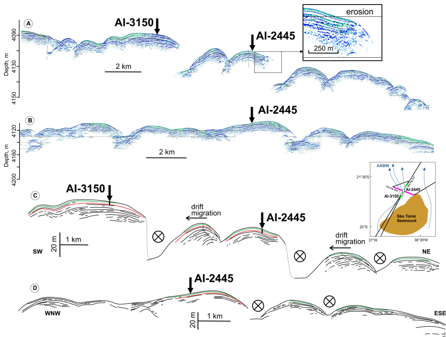
Figure 5. Fragments of seismic profile AI-37 (with interpretation). Red solid line indicates seismic reflector corresponding to coarse grained layer recovered in the lower parts of the sediment cores. Green solid line marks seismic reflector corresponding to the layer of foraminiferal sand in cores AI-3150 and AI-2445. Seismic evidence of erosion is presented in the upper right insert. Suggested direction of bottom currents near the São Tomé Seamount is shown in the lower right insert. Location of seismic lines is shown in Figure 1B. Core lithology is presented in Figure 6.
