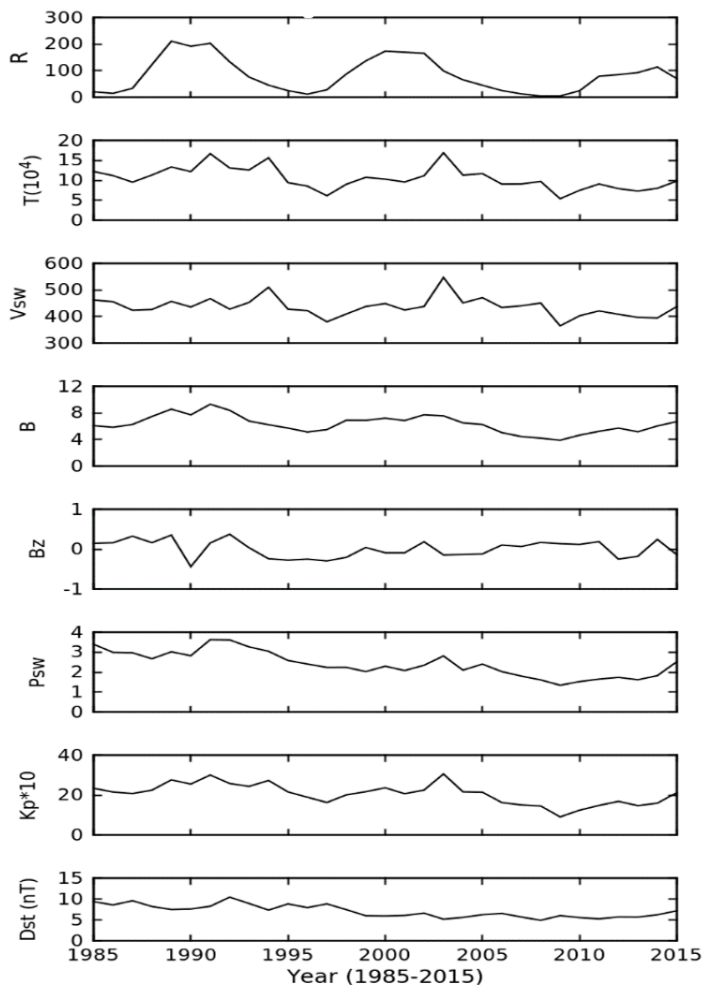
Figure 1. Yearly values of sunspots number ( R ), Solar wind velocity ( V_{sw} ), Magnitude of magnetic field ( B ), North-south component of interplanetary magnetic field ( B_z ), Solar wind Plasma Pressure ( P_{sw} ), K_p and Dst indices from 1985–2015.
