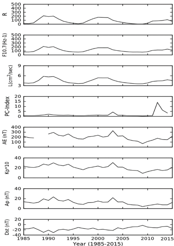
Figure 2. Yearly values of sunspots number ( R ), solar flux ( F_{10.7} ), Lyman Alpha ( L ), PC, AE, K_p , A_p and Dst indices for the same periods from 1985–2015.
