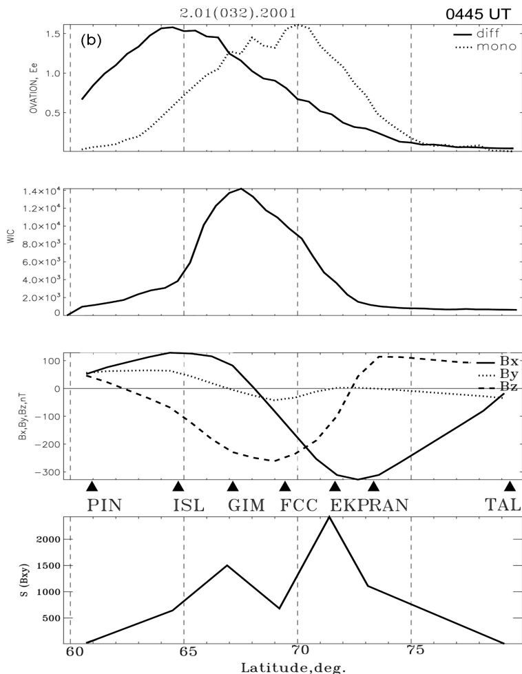
Figure 9b. The same format as in Figure 9a, but for \Lambda = 325.5^\circ , UVI image at 0444:20 UT, magnetic field disturbance as compared with reference field at 0437 UT estimated for the period 0443 UT \pm 2.5 min (third panel), and Pi2 power during 0445 UT \pm 7.5 min.
