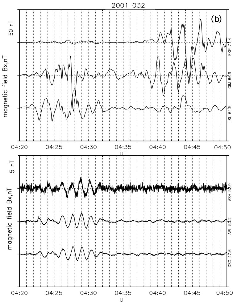
Figure 7b. Magnetograms of X component geomagnetic field variations at the high-latitude CARISMA stations (upper panel) and at the mid-latitude MEASURE stations (bottom panel) on 02/01, 2001 (day 032) 0420–0450 UT. CGM latitudes are indicated near station codes.
