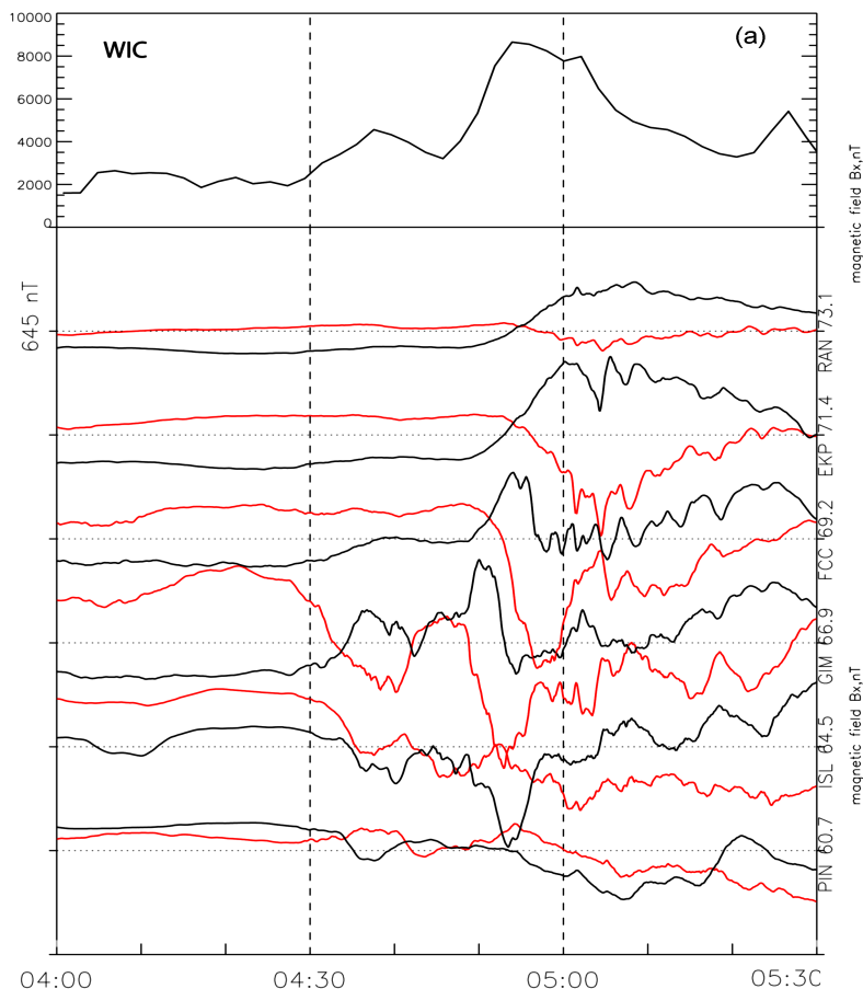
Figure 3a. Upper panel: Time evolution of UV WIC intensity from IMAGE spacecraft (integrated over the latitudinal range \Delta\Phi = 60.7^\circ - 73.1^\circ ) above the geomagnetic meridian 330^\circ . Lower panel: magnetograms of X component (red line) and Z component (black line) geomagnetic field variations along the latitudinal profile \sim 330^\circ on 12/23, 2000 (day 358) 0400–0530 UT. CGM latitudes are indicated near station codes. The scale between ticks is shown near
