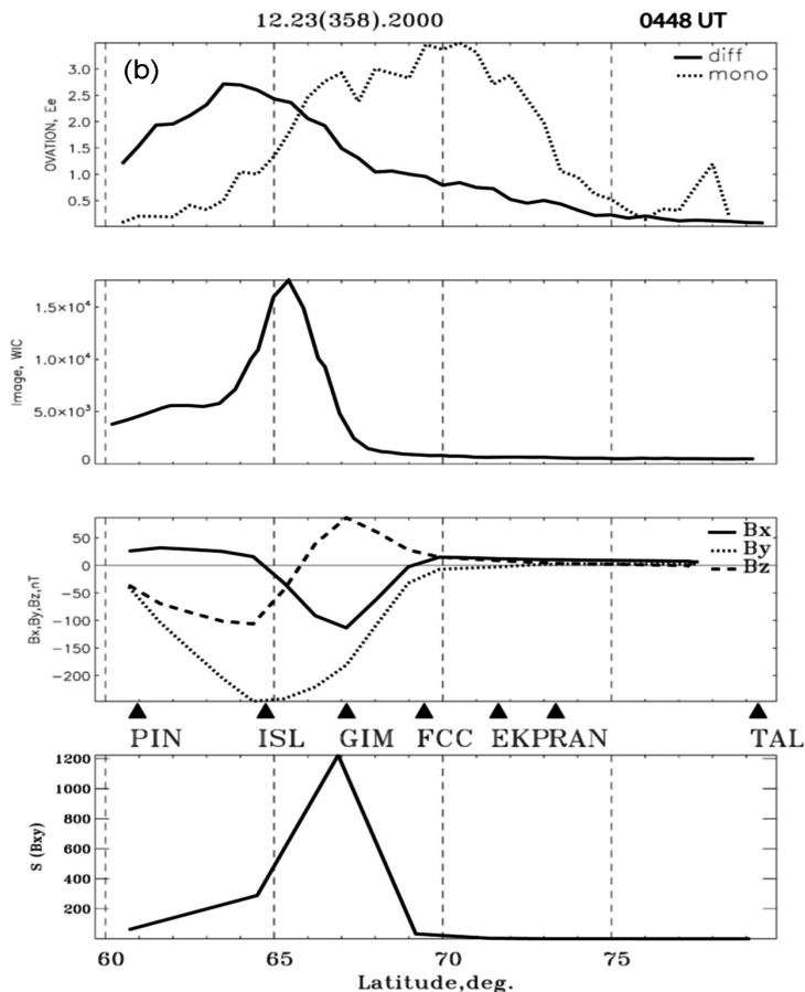
Figure 5b. The same format as in Figure 5a, but for the OVATION-prime model on 0448 UT, WIC on 0447:47 UT along \Lambda = 346.8^\circ , magnetic field disturbance along the \sim 330^\circ profile as compared with reference value at 0445 UT estimated for the period 0456 UT \pm 2.5 min, and Pi2 power recorded during the time interval 0448 UT \pm 2.5 min.
