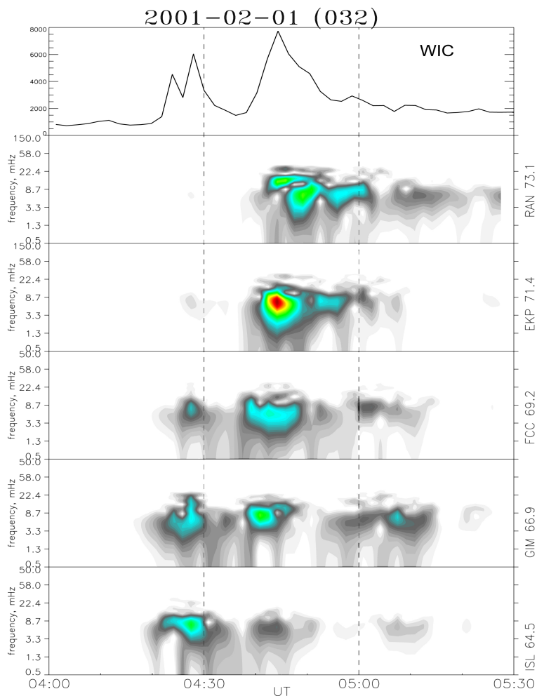
Figure 8. Time evolution of integrated UV auroral intensity (upper panel) and dynamic spectra of geomagnetic fluctuations in the Pi2 band (5–30 mHz) along the latitudinal CARISMA profile \sim 330^\circ on 02/01, 2001 (day 032) 0400–0530 UT.
