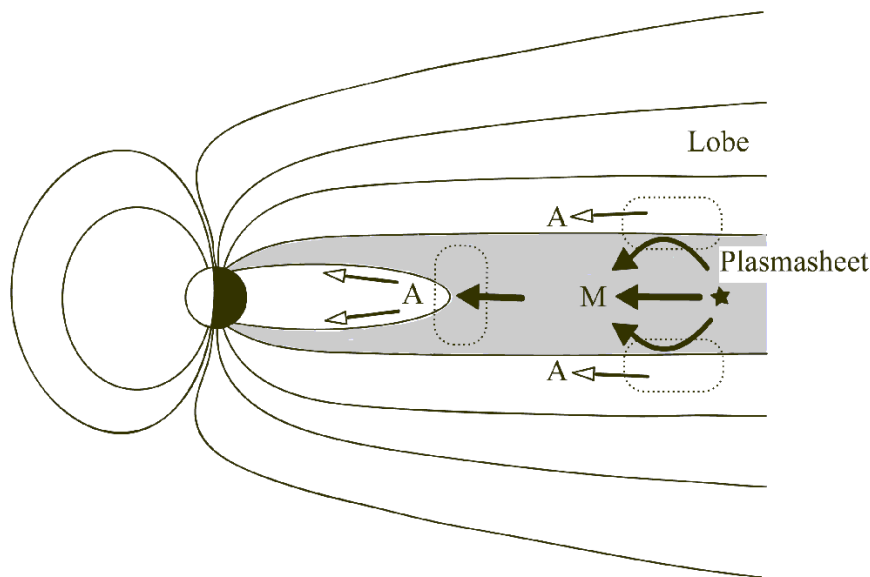
Figure 11. Schematic illustration of the ULF wave energy propagation channels from the substorm origin (“tailquake” marked by black star) to the Earth’s ionosphere via Alfvenic (A) or fast magnetosonic (M) modes. Dotted lines indicate region of the mode conversion.
