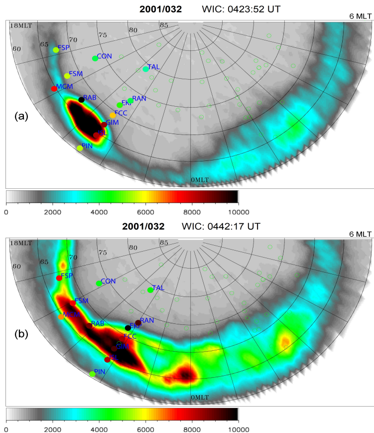
Figure 6. (a) An image of the auroral UV activation observed by the WIC instrument on the IMAGE spacecraft ( L -filter) on 2001, 02/01 (day 032) at 0423:52 UT. The relative Pi2 signal power (estimated within a time interval of \pm 2.5 min from 0425 UT) and UV intensity are color coded. The maximal disturbances are B_{\max} = 49.0 dB, UVI_{\max} = 21,457 r.u. (b) The same format as in top panel. The WIC snapshot is taken at 0442:17 UT, and the Pi2 signal power with B_{\max} = 46.0 dB has been estimated within a time interval 0445 \pm 0007:30 UT. The maximal disturbance of UVI_{\max} = 11,994 r.u.
