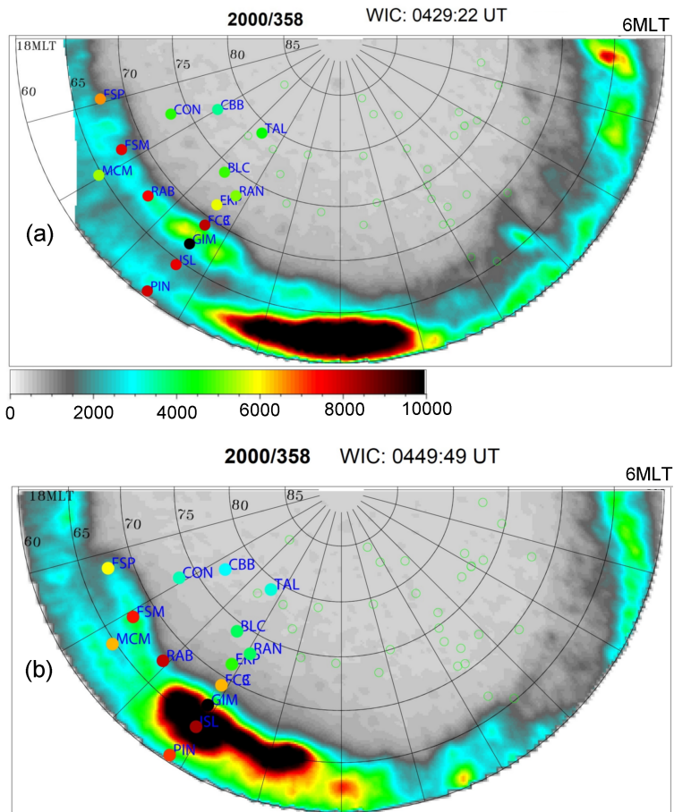
Figure 2. (a) An image of the auroral UV activation observed by the WIC instrument on the IMAGE spacecraft on 2000, 12/23 (day 358) at 0429:22 UT. The relative Pi2 signal power (estimated within a time interval of from 0430 \pm 2.5 min UT) and UV intensity are color coded. The maximum power of Pi2 horizontal component B_{\max} = \sqrt{X^2 + Y^2} = 14.7 dB, maximum of UV intensity UVI_{\max} = 23,900 (relative units). (b) The same but for UV image on 0449:49 UT. The Pi2 signal power B_{\max} = 52.0 dB is estimated for time interval 0448 \pm 2.5 min UT. The maximal disturbances are characterized by UVI_{\max} = 22,689 r.u.
