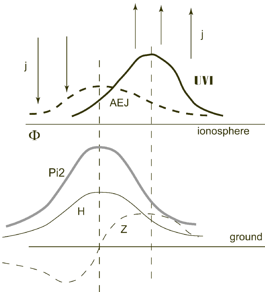
Figure 12. The relative locations of the latitudinal profile of the Pi2 power, auroral electrojet (AEJ), auroral UV luminosity, and ground magnetic bay ( H and Z components).
