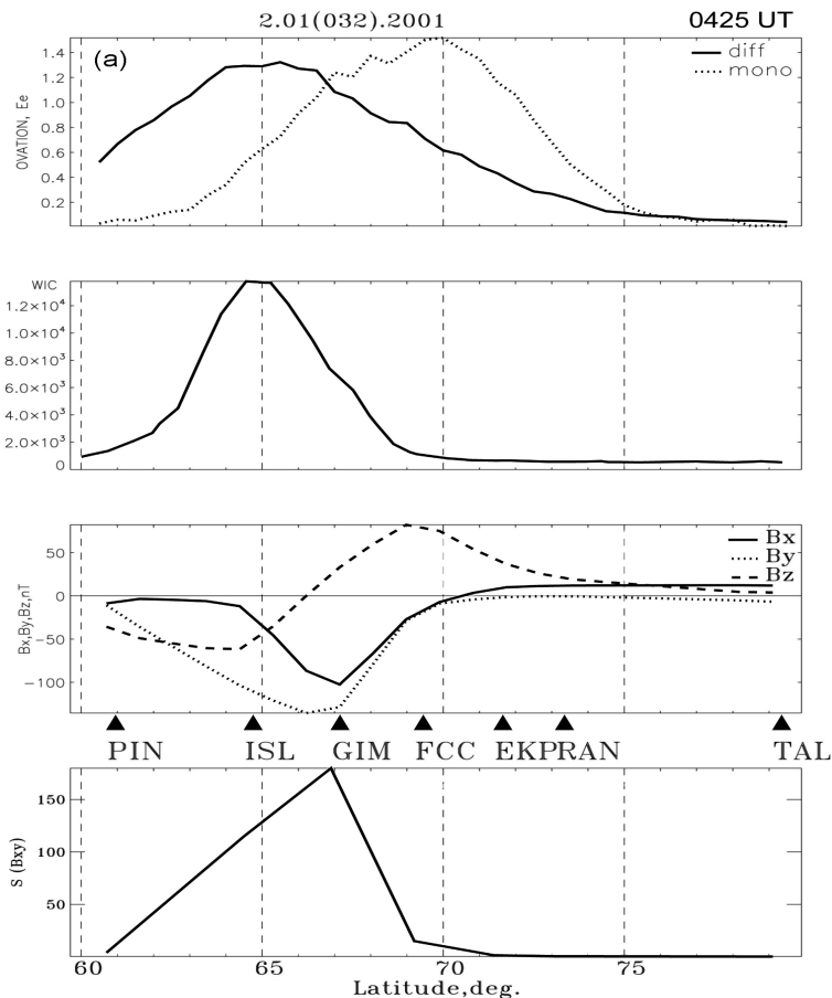
Figure 9a. Latitudinal distribution on 2001, 02/01 (day 032) of the particle precipitation zones as derived from the OVATION-prime model (upper panel); WIC intensity along the longitude \Lambda = 317.5^\circ on 0425:55 UT (upper panel), magnetic field disturbance (solid line – X component; dashed line – Z component; dotted line – Y component) along \sim 330^\circ profile as compared with reference field at 0425 UT estimated for the period 0428 UT \pm 2.5 min (third panel), and Pi2 power in the 5–30 mHz band (bottom panel) taken during the time interval around auroral activation (0430 UT \pm 2.5 min).
