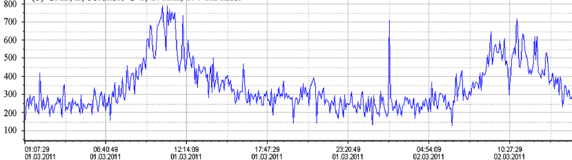
(b) GAE, Z, borehole G-1, 1012m, 150 Hz filter
